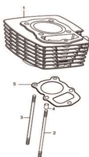
Fig.2 CILINDRO DO MOTOR (P05-C020-0008)
