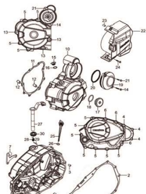
Fig.4 TAMPAS LATERAIS DO MOTOR(P05-C040-0012)
