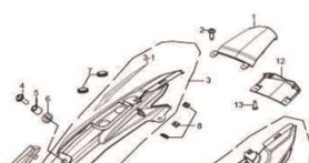
Fig.40 TAMPAS LATERAIS TRASEIRAS (P05-C390-0001)
