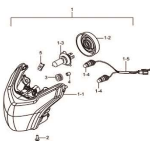
Fig.23 FAROL (P05-C220-0001)
