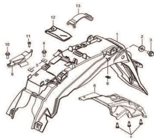
Fig.36 PARALAMA TRASEIRO (P05-C350-0001)
