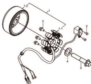
Fig.19 MAGNETO (P05-C180-0002)
