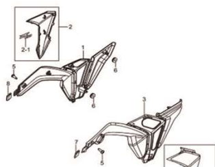
Fig.32 TAMPAS DO CHASSI (P05-C310-0011)
