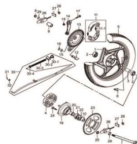
Fig.48 RODA TRASEIRA (P05-C460-0003)
