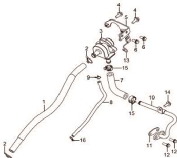
Fig.13 VALVULA DE AR 2ND (P05-C120-0003)
