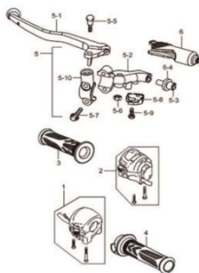
Fig.35 MANETES E MANOPLAS (P05-C340-0005)
