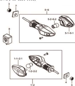
Fig.24 SETAS (P05-C230-0003)
