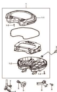
Fig.22 VELOCIMETRO (P05-C210-0001)
