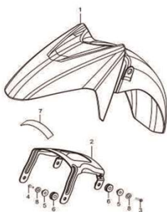
Fig.33 PARALAMA FRONTAL (P05-C320-0001)
