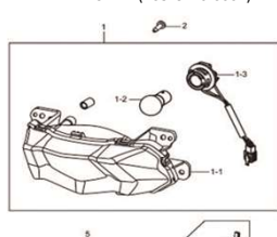
Fig.25 LAMTERNA TRASEIRA (P05-C240-0002)
