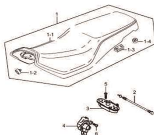
Fig.39 ASSENTO (P05-C380-0001)
