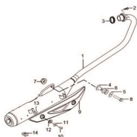
Fig.12 ESCAPAMENTO (P05-C110-0009)
