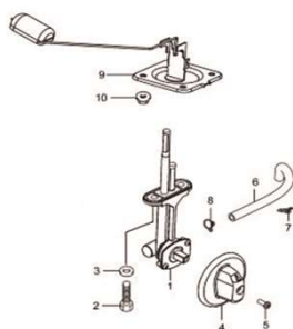
Fig.31 REGISTRO DE COMBUSTIVEL (P05-C300-0002)
