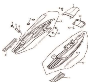
Fig.40 TAMPAS LATERAIS TRASEIRAS (P05-C390-0001)
