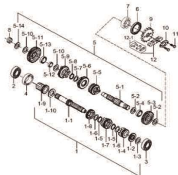
Fig.16 CAMBIO (P05-C150-0007)
