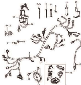
Fig.26 CHICOTE (P05-C250-0007)
