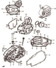
Fig.4 TAMPAS LATERAIS DO MOTOR(P05-C040-0012)
