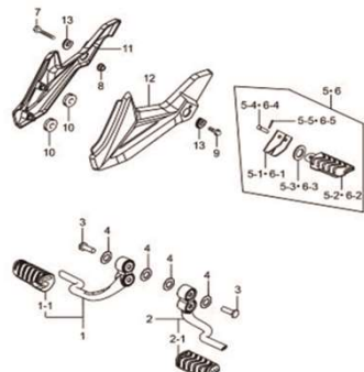
Fig.29 PADALEIRA (P05-C280-0001)
