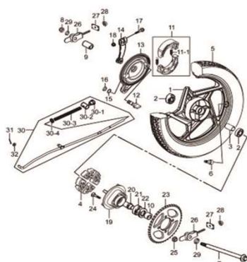
Fig.48 RODA TRASEIRA (P05-C460-0003)
