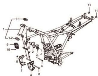
Fig.27 CHASSI (P05-C260-0016)
