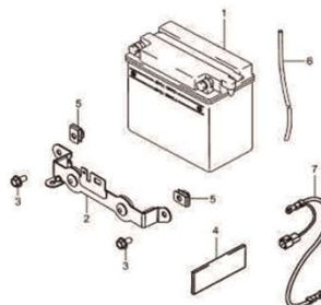
Fig.20 BATERIA (P05-C190-0003)
