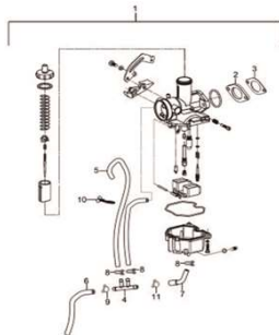
Fig.9 CARBURADOR (P05-C090-0005)
