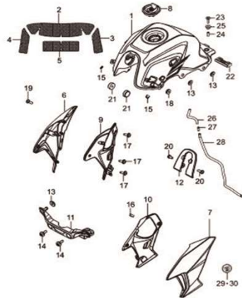
Fig.30 TANQUE DE COMBUSTIVEL (P05-C290-0008)
