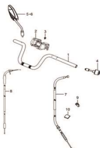
Fig.34 GUIDÃO (P05-C330-0007)
