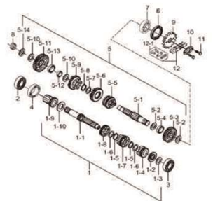
Fig.16 CAMBIO (P05-C150-0007)
